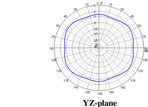
Figure 7 Radiation pattern of the proposed antenna at resonant frequency of 2689 MHz.
