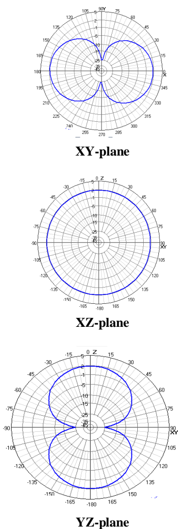
Figure 6 Radiation pattern of the proposed antenna at resonant frequency of 944 MHz.
