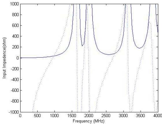
Figure 4 Input impedance characteristics of Hybrid Koch fractal antenna.
