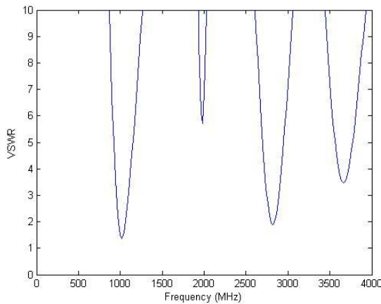
Figure 5 VSWR characteristics of Hybrid Koch fractal antenna
