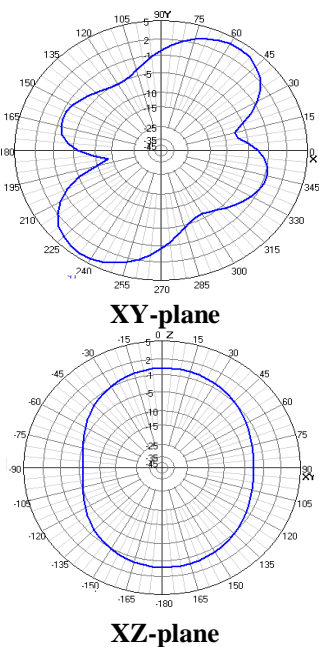
Figure 6 Radiation pattern of the proposed antenna at resonant frequency of 944 MHz.
